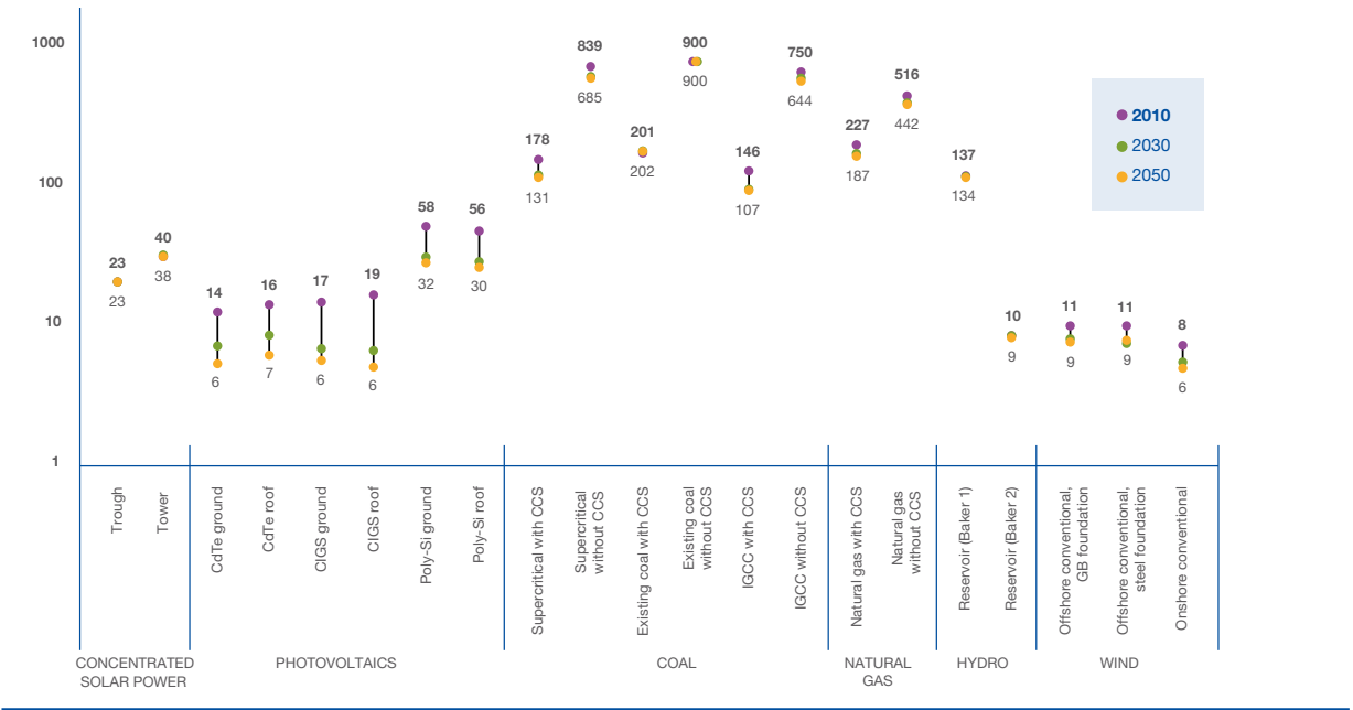
Figure 1: Life-cycle GHG emissions of different energy technologies, in gCO 2 e/kWh, reflecting application of the technology in Europe 12 . The numbers for future years reflect a reduction of emissions expected due to technical progress and the reduced emissions in the production of equipment following the implementation of a mitigation scenario.
