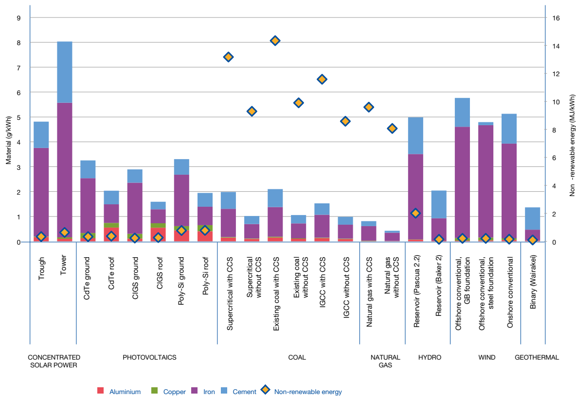
Figure 5: Bulk material and non-renewable energy requirements per unit power produced. 28
