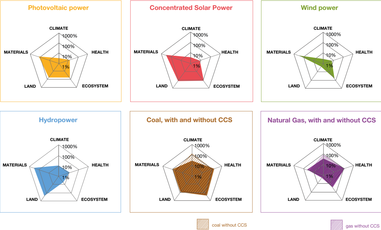
Figure 7: An overview over the life cycle results of different technology groups compared to the global average mix of electricity production technologies. The indicators are the use of the bulk materials (cement, iron and steel, copper, and aluminium), land occupation, greenhouse gas emissions, and the endpoint indicators for human health and ecosystems (excluding the contributions of climate change and land use, but including the production of materials.)
