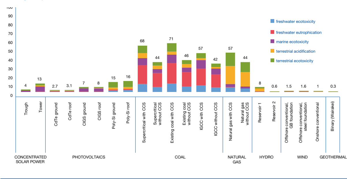
Figure 3: Ecosystem impacts in species-year affected per 1000 TWh of electricity following different damage pathways, reflecting Europe 2010 23 .
