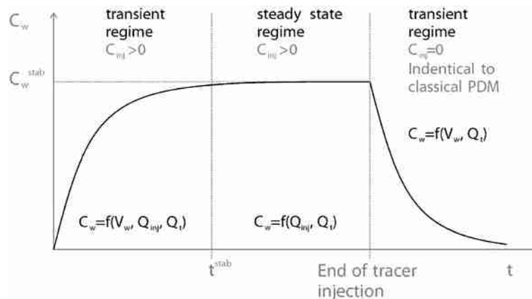
Fig. 1. Evolution of tracer concentrations ( C_w ) in a well where a FVPDM is performed. The steady state regime is reached when the mass flux of tracer injected in the well equilibrate with the mass flux of tracer flushed out of the well by the groundwater flow that transit by the well screen. The experiment ends as a classical PDM when the injection of tracer is stopped.
